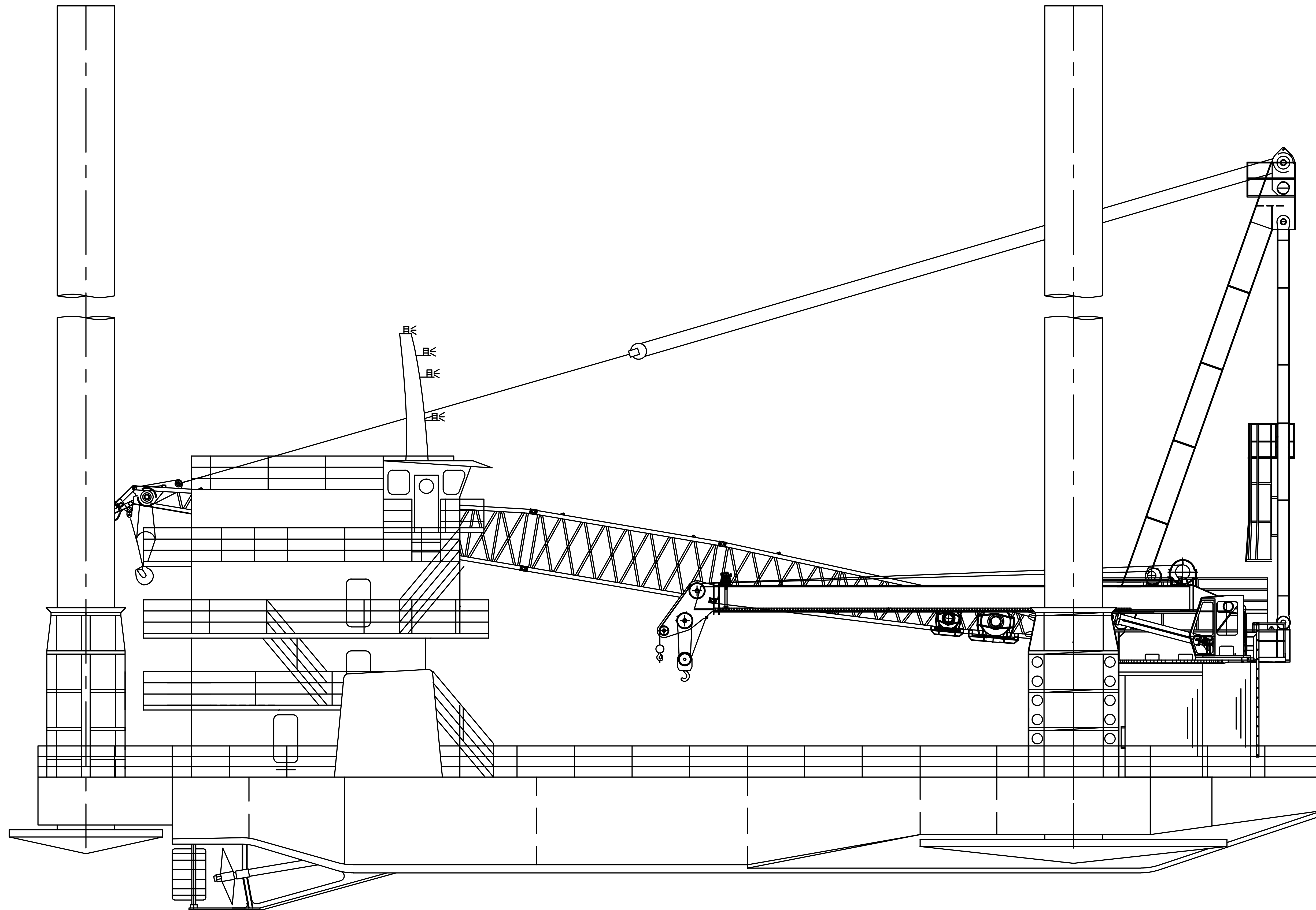
DMI CLASS 215 LIFTBOAT OUTBOARD PROFILE
