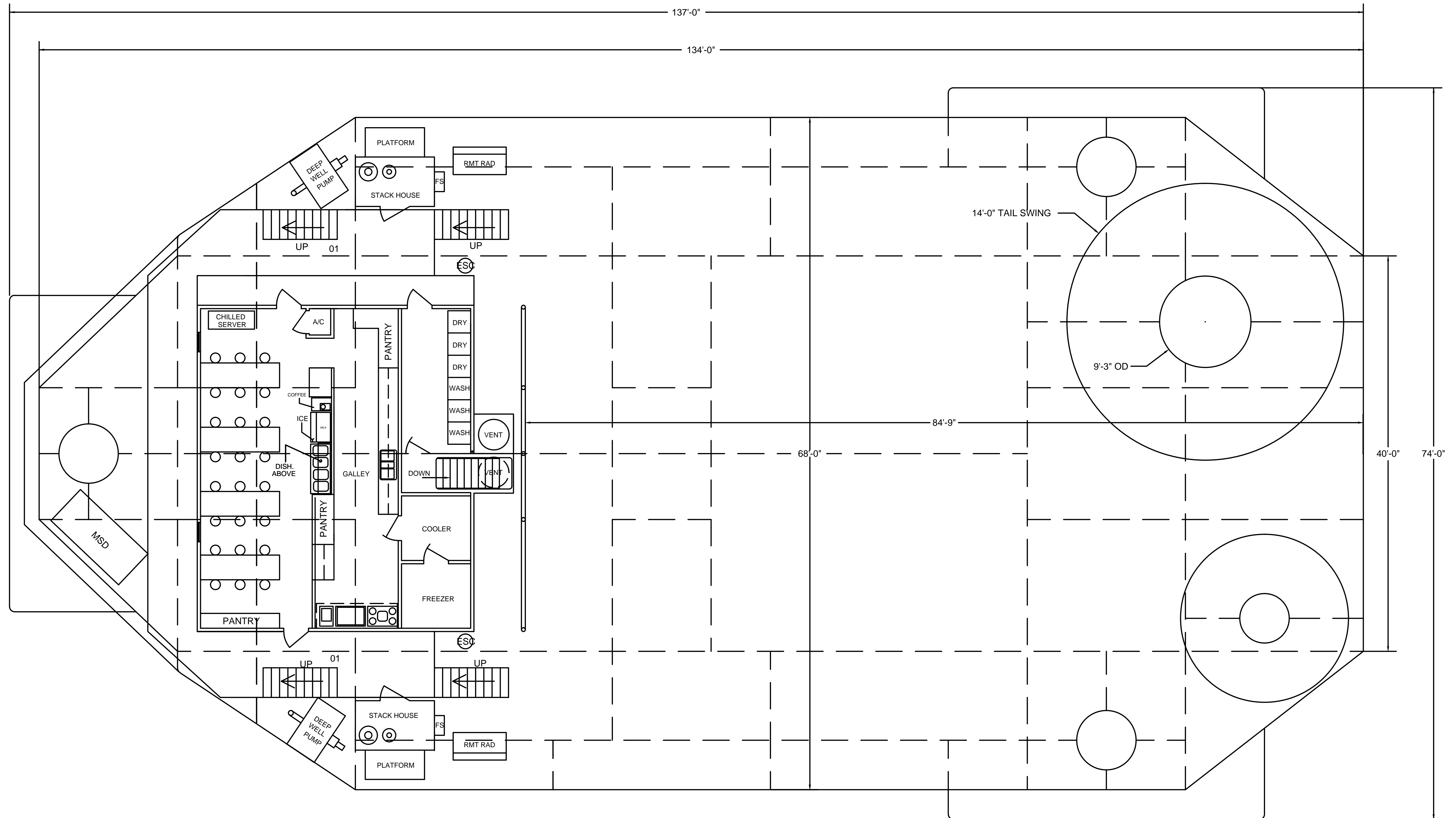
DMI CLASS 215 LIFTBOAT GENERAL ARRANGEMENT - MAIN DECK
