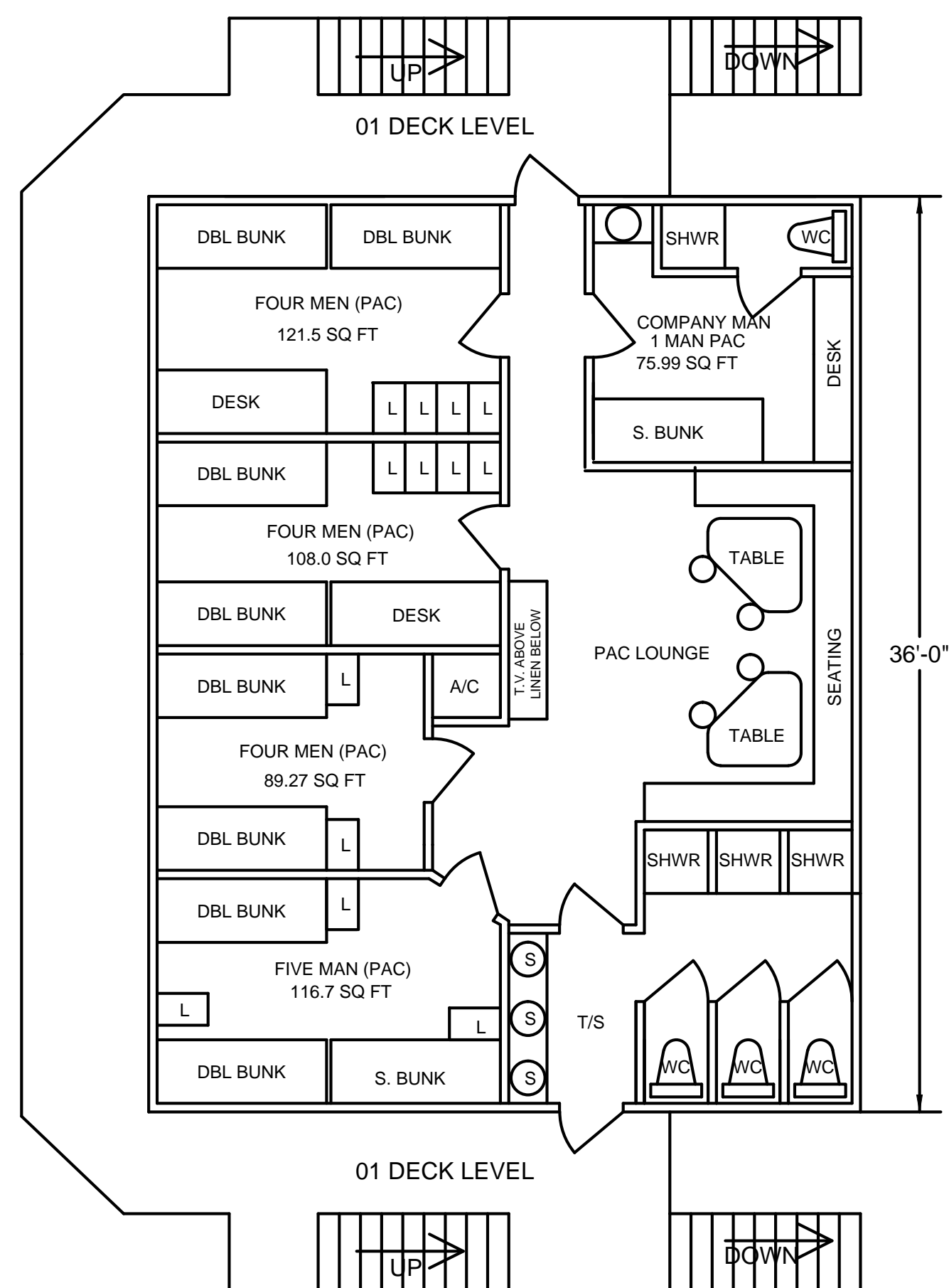
DMI CLASS 215 LIFTBOAT GENERAL ARRANGEMENT - LEVEL 01
