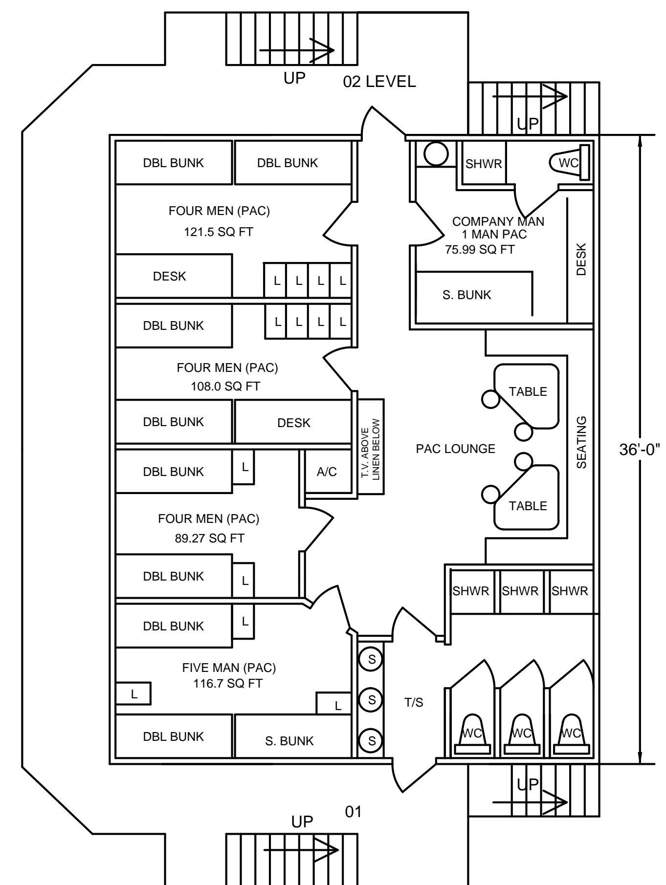
DMI CLASS 215 LIFTBOAT GENERAL ARRANGEMENT - LEVEL 02
