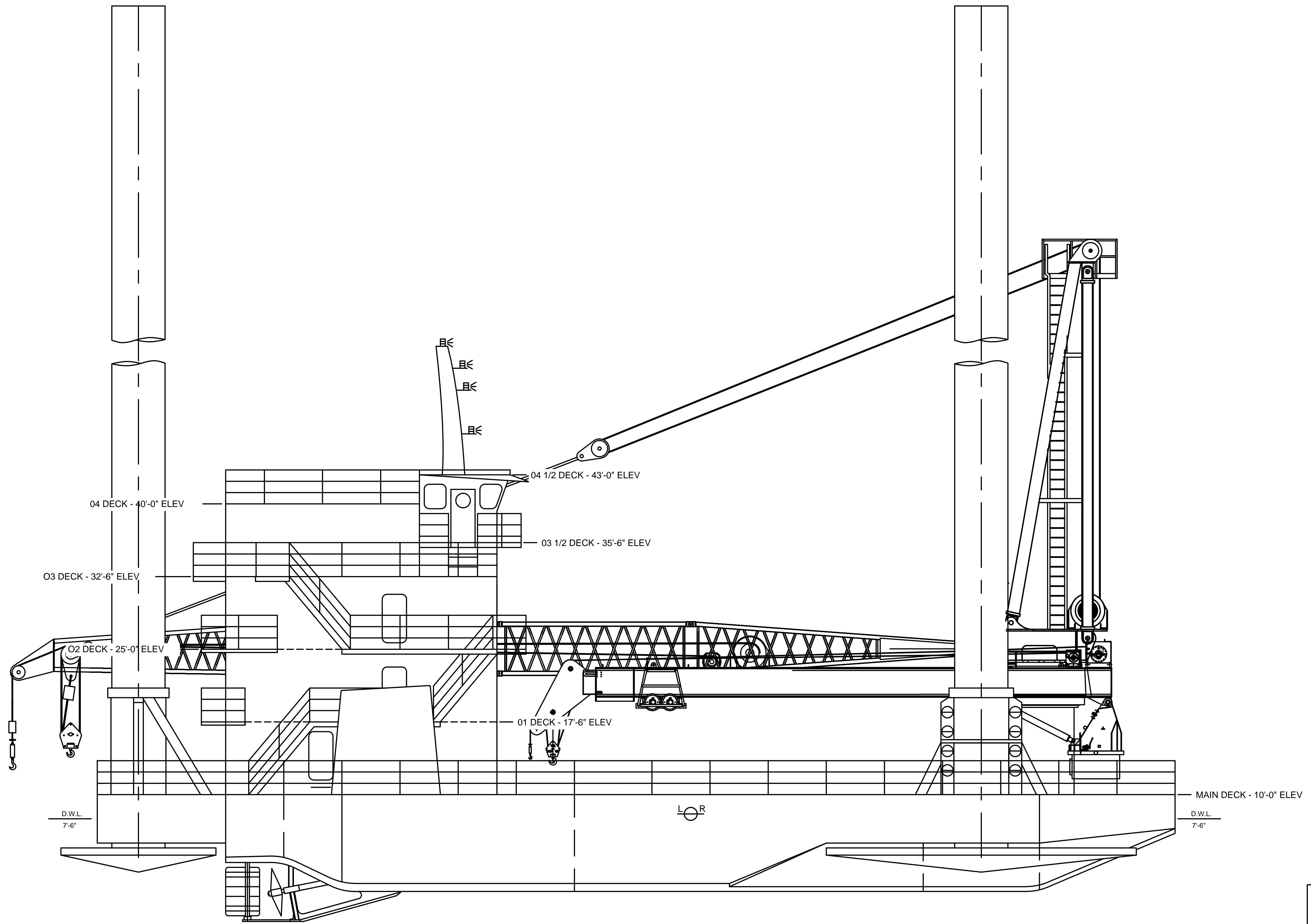
DMI CLASS 200 LIFTBOAT OUTBOARD PROFILE
