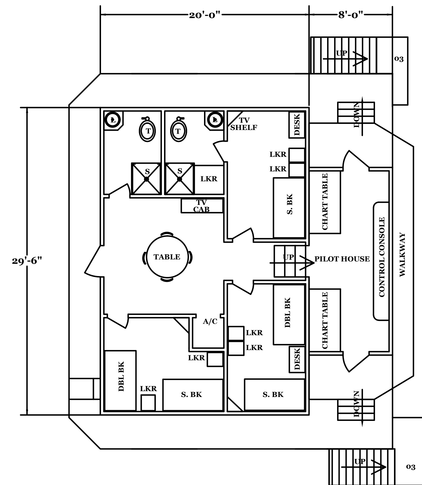
CLASS 200 LIFTBOAT GENERAL ARRANGEMENT - LEVEL 03
