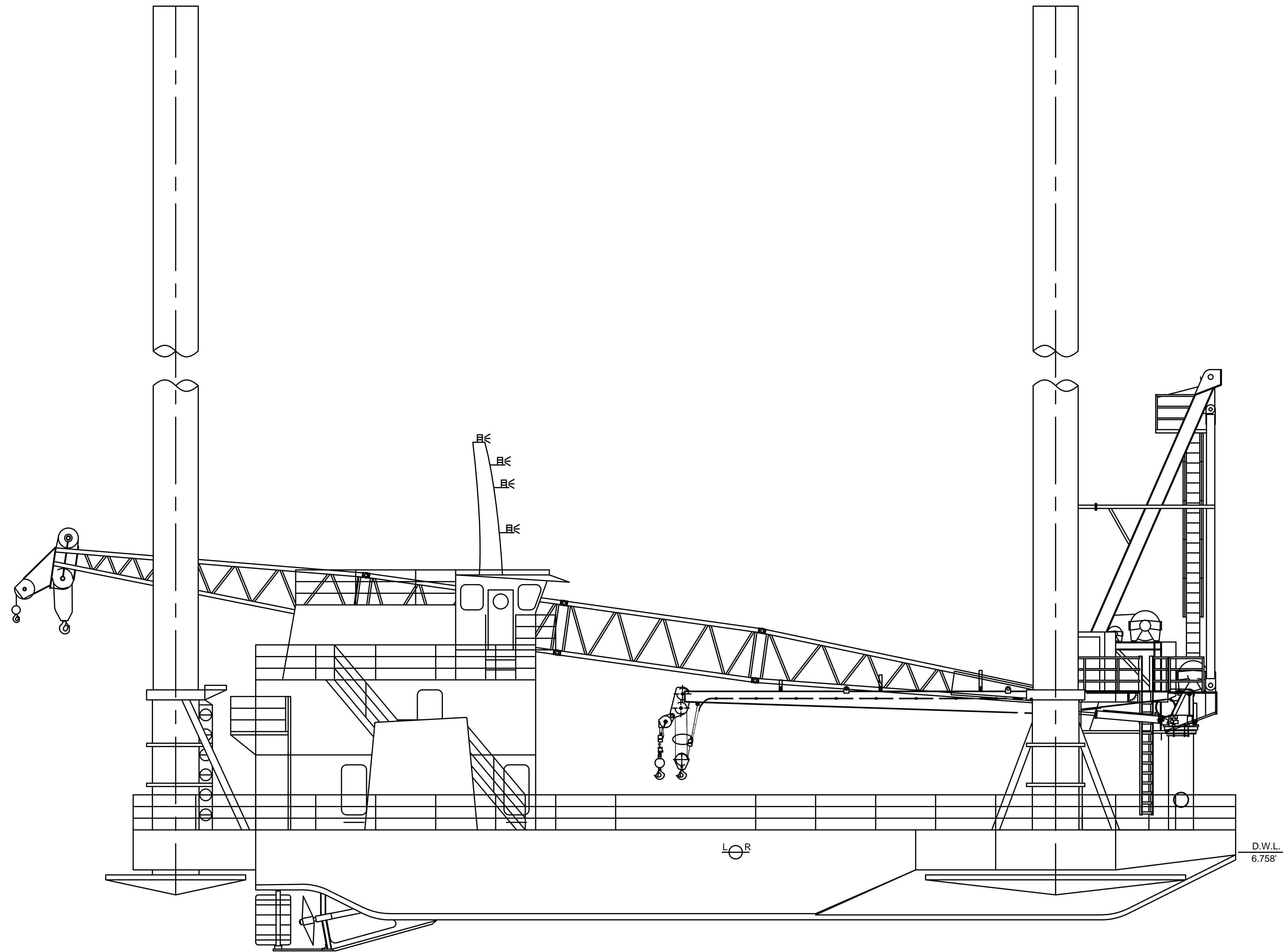
DMI CLASS 175 LIFTBOAT OUTBOARD PROFILE
